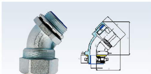
TYPE ZGHM (外螺紋接頭45°)
